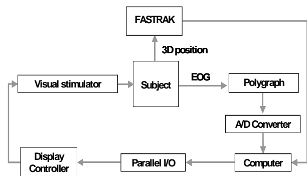
Fig. 1 Block diagram of the experimental system
